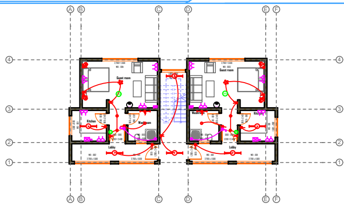
FIRST FLOOR LAYOUT SCALE 1:100
