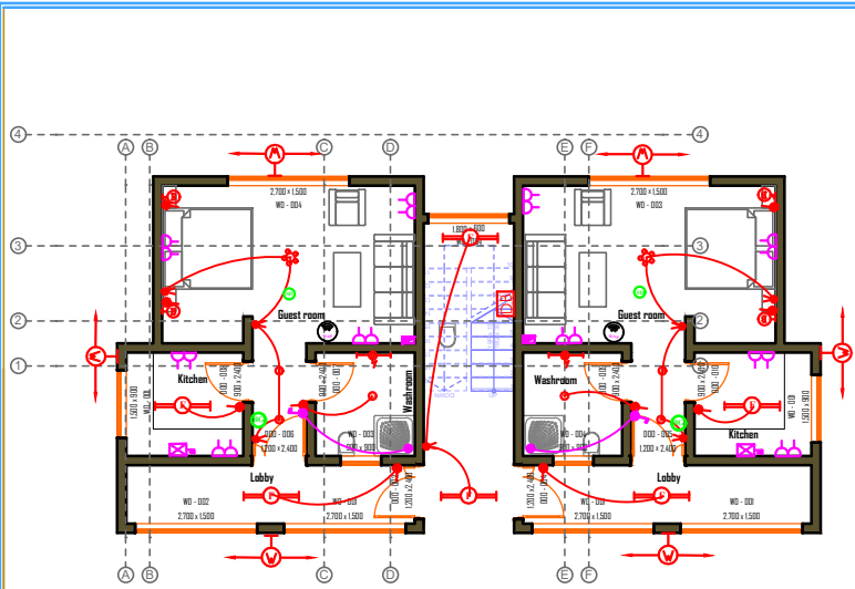
GROUND FLOOR LAYOUT SCALE 1:100
