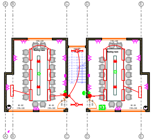
SECOND FLOOR LAYOUT SCALE 1:100
